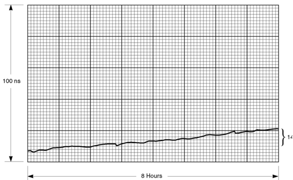
Figure A-8. Error Measurement
