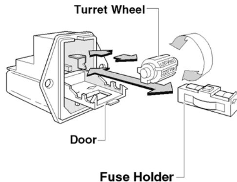
Figure 7-1. Line Voltage Fuse Selection with Power Module Turret Wheel
